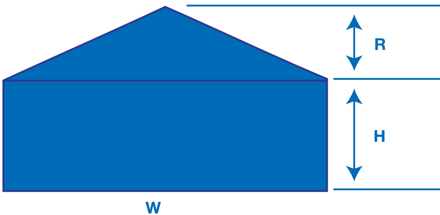
Figure 112: Elevation of house showing height (H), width (W), roof (R) for calculating cross section area for tunnel ventilation calculations.
