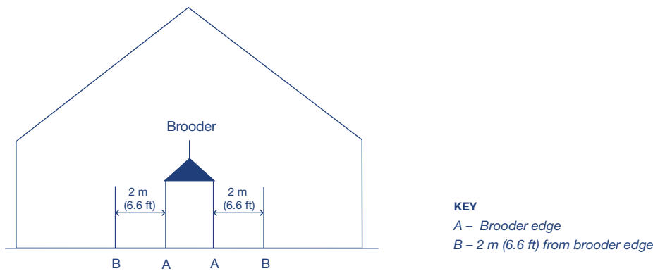
Figure 15: Spot brooding temperature gradients.
