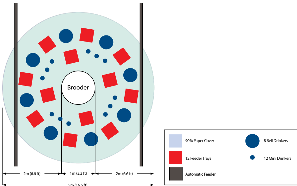
Figure 9: Example of a typical spot brooding layout (1,000 chicks).
