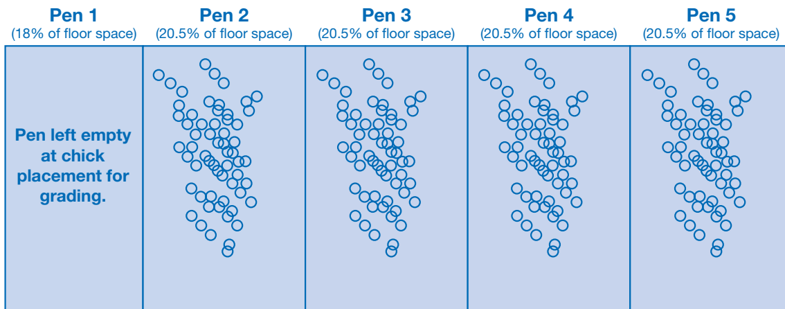
Figure 33: Pre-grade house set up for a 3-way grade with adjustable penning.
