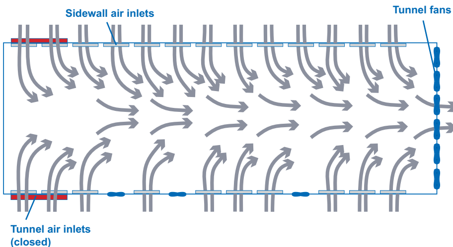
Figure 109: Typical air movement during transitional ventilation.
