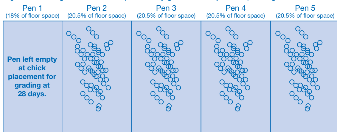
Figure 29: Pre-grade house set up for 2-way grade with adjustable penning.
