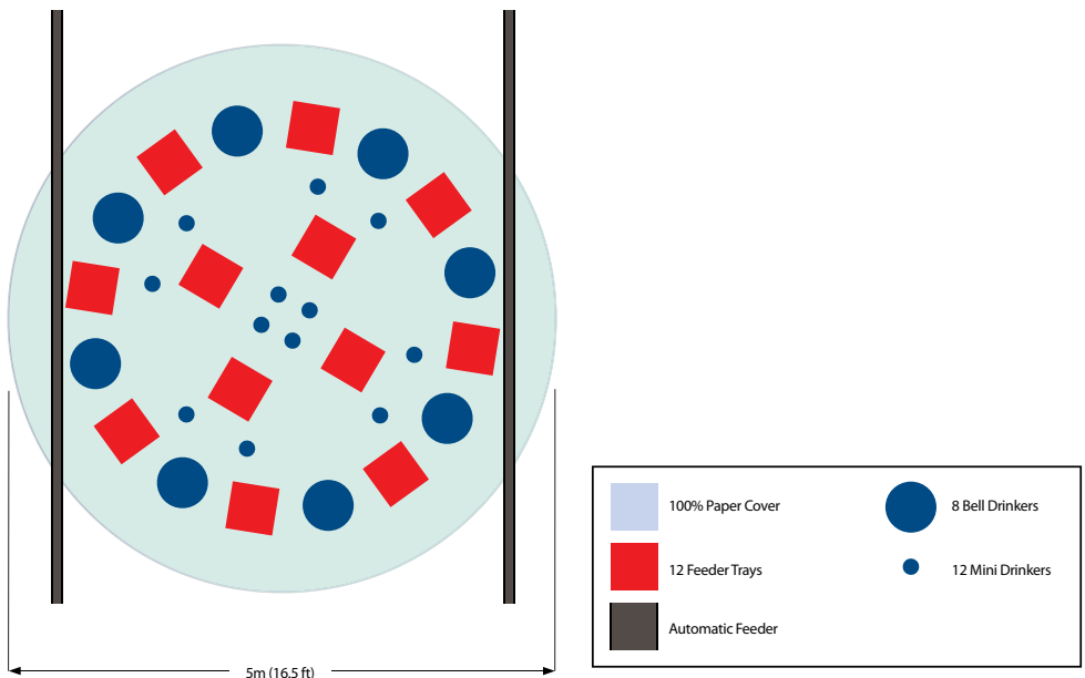
Figure 11: Typical whole-house brooding layout for 1,000 chicks. In this situation, chicks are placed in a brooder surround.
