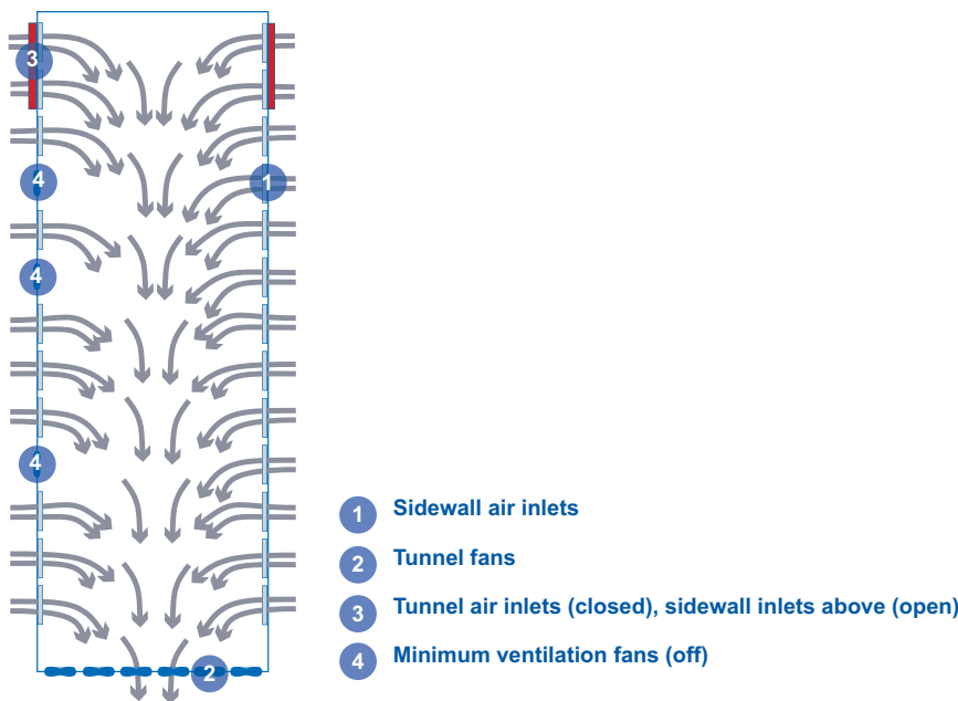
Figure 6.11: Typical air movement during transitional ventilation. In this example sidewall fans are off.
