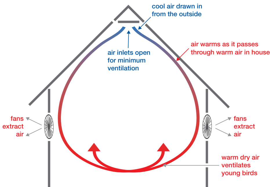
Figure 6.16: Diagram of reverse flow (roof inlet) ventilation.
