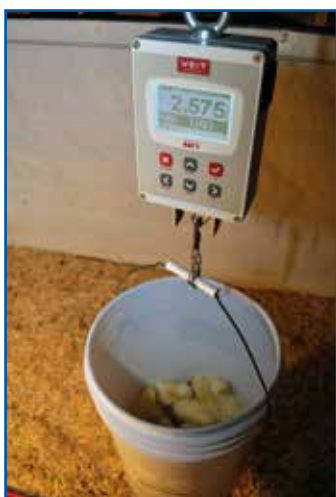
Figure 7.2: Manual bulk weighing of chicks with an electronic scale.
