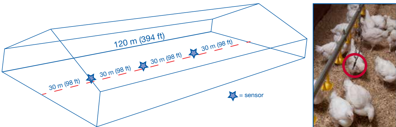
Figure 2.9: Correct location for temperature and humidity sensors.
