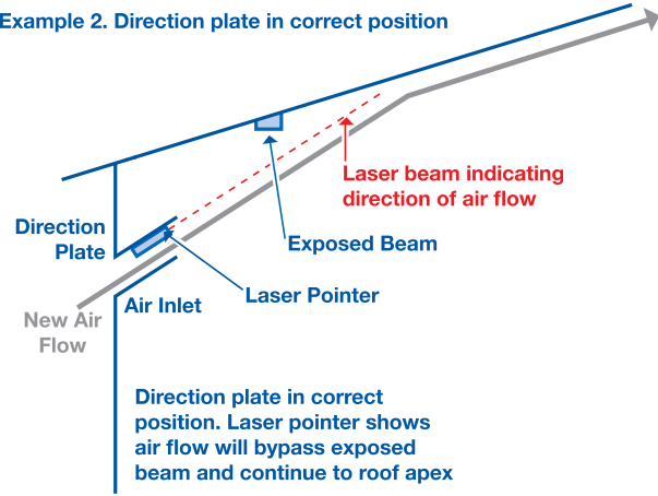
Example 2. Direction plate in correct position
