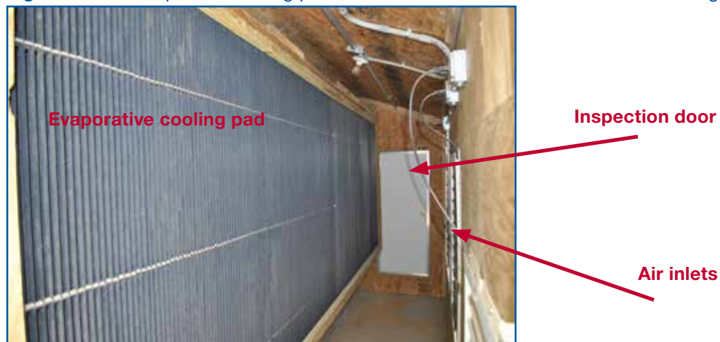
Figure 6.20: Example of a cooling pad installed on the sidewall of the house in a doghouse.
