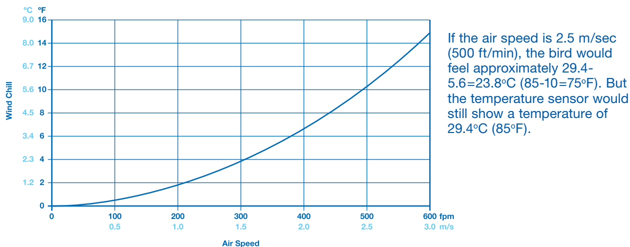
Figure 6.15: Theoretical cooling effect felt by a 3.5 kg (7.7 lb) broiler at an air temperature of 29.4°C (85°F).
