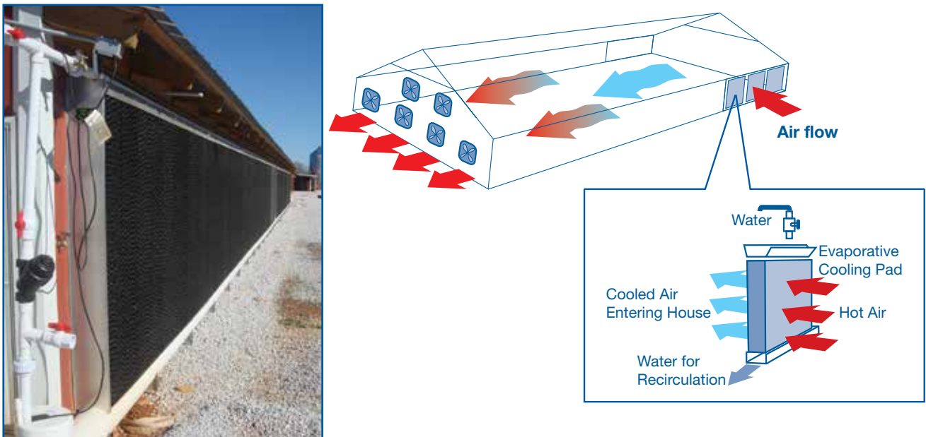
Figure 6.19: Pad cooling with tunnel ventilation.
