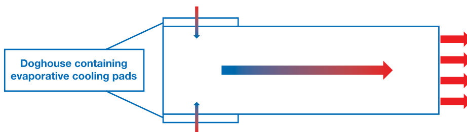
Figure 6.12: Air flow in a tunnel ventilation house.
