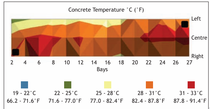
Excellent uniformity of concrete temperature
