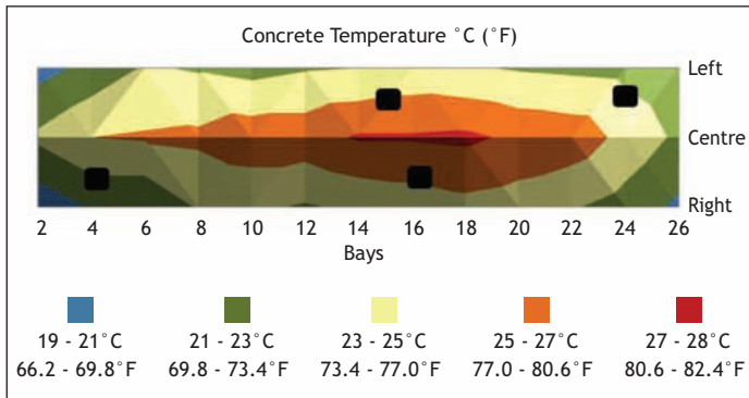
Poor uniformity of concrete temperature
