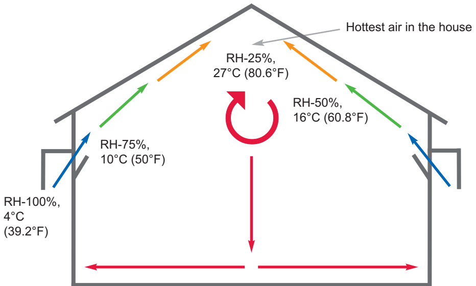
Ideal air flow for negative ventilation
