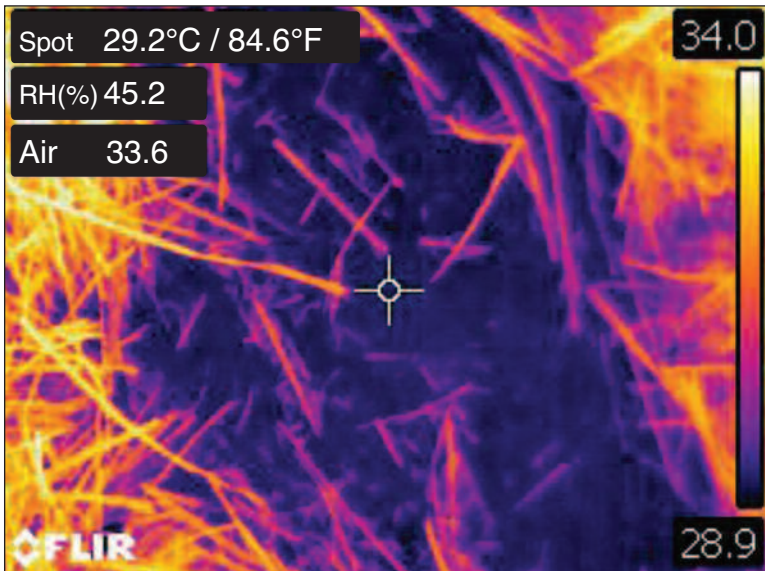
Example of good concrete temperature from adequate pre-heating and uniform distribution of heat by the minimum ventilation system
