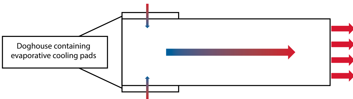
Figure 6.12: Air flow in a tunnel ventilation house.
