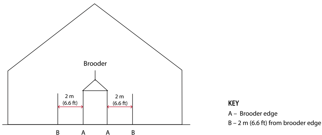
Figure 2.5: Spot brooding - areas of temperature gradients
