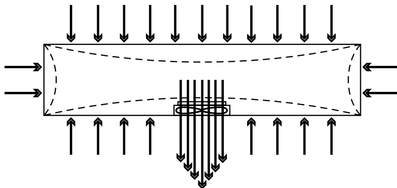
Figure 6.4: Diagram illustrating airflow through air inlets in negative pressure system.
