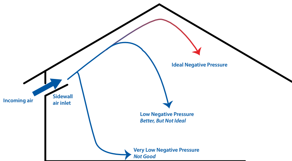
Figure 6.5: Using negative pressure to control air speed.
