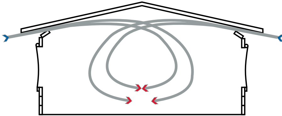
Figure 6.6: Correct airflow during minimum ventilation.
