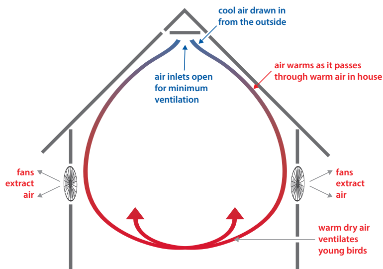
Figure 6.16: Diagram of reverse flow (roof inlet) ventilation.
