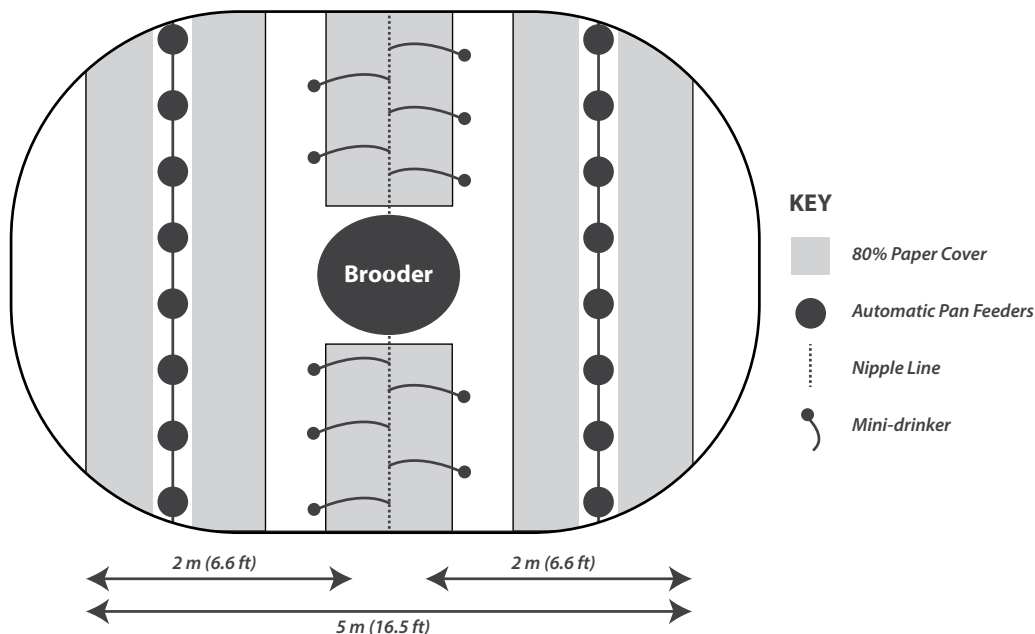
Figure 2.4: Typical spot brooding layout (1,000 chicks).
