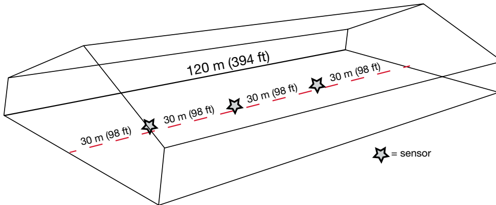
Figure 2.9: Correct location for temperature and humidity sensors.
